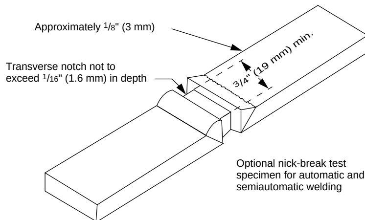
Figure 5—Nick-Break Test Specimen
