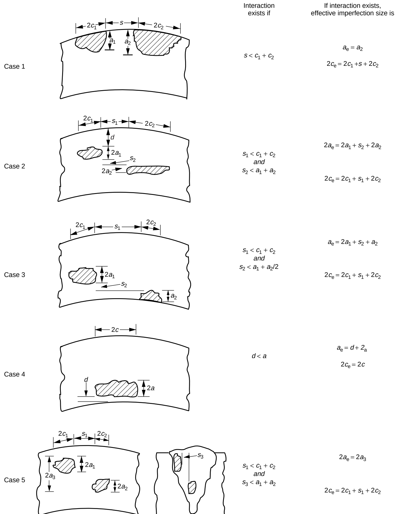
Figure A-6—Criteria for Evaluation of Imperfection Interaction
