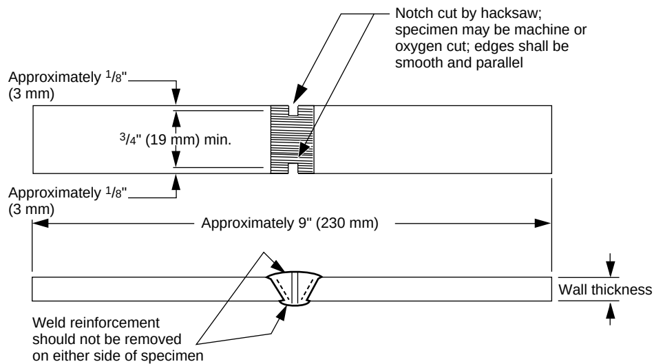
Figure 4—Tensile-Strength Test Specimen
